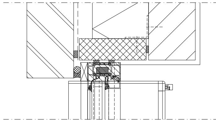
Principedetail
