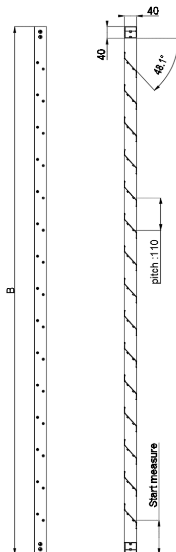
SECTION
