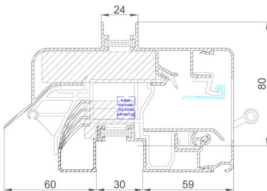
GlasMax 'ZR' – glasgoot 30 mm
