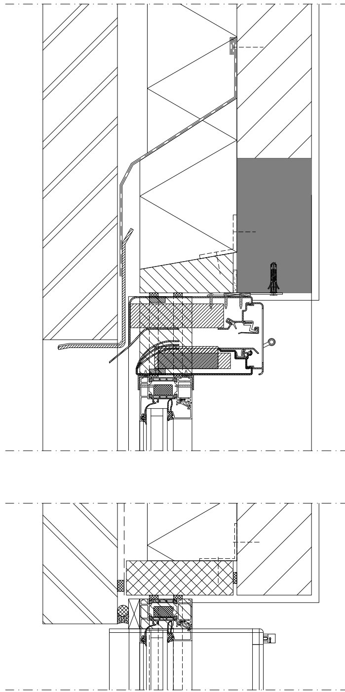
Principle sketch
