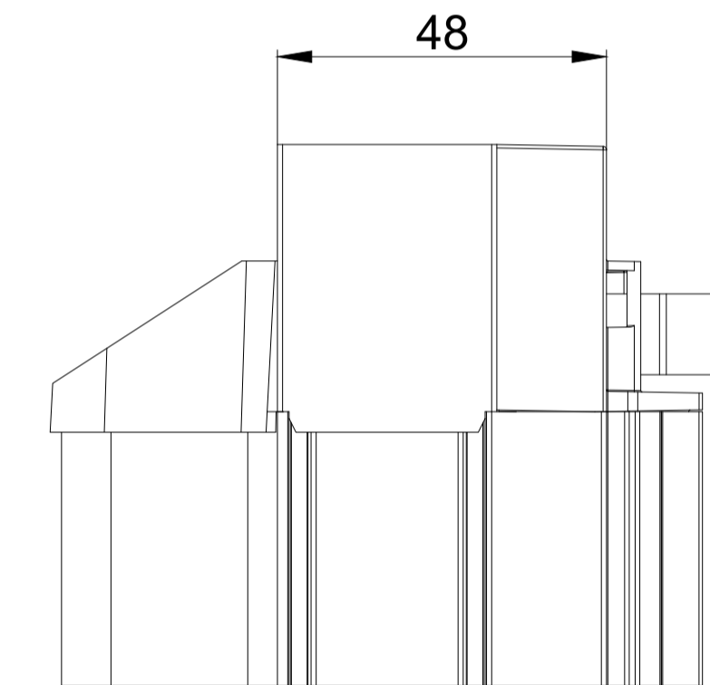
DucoKlep 80 ZR / GG54
