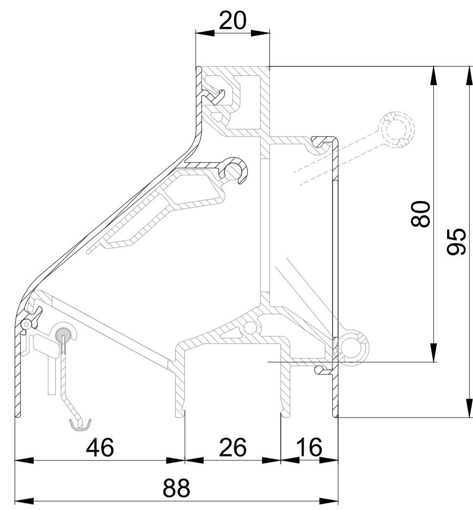
DucoLine 10-17-23 'ZR' / GG26
