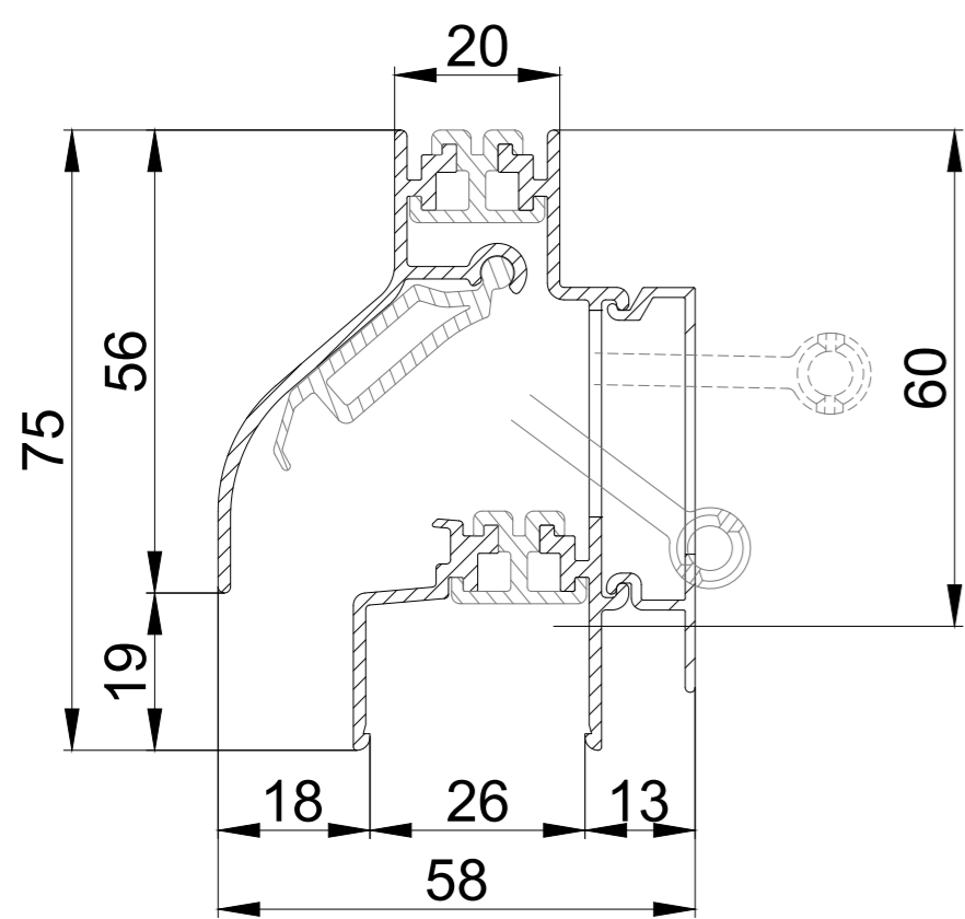
DucoSmart 60 / GG26
