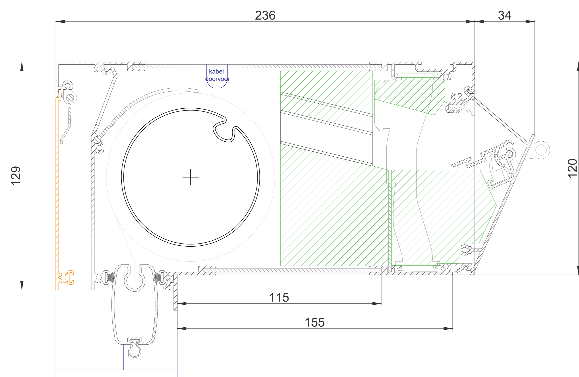
DucoTwin 120 Alto ZR
