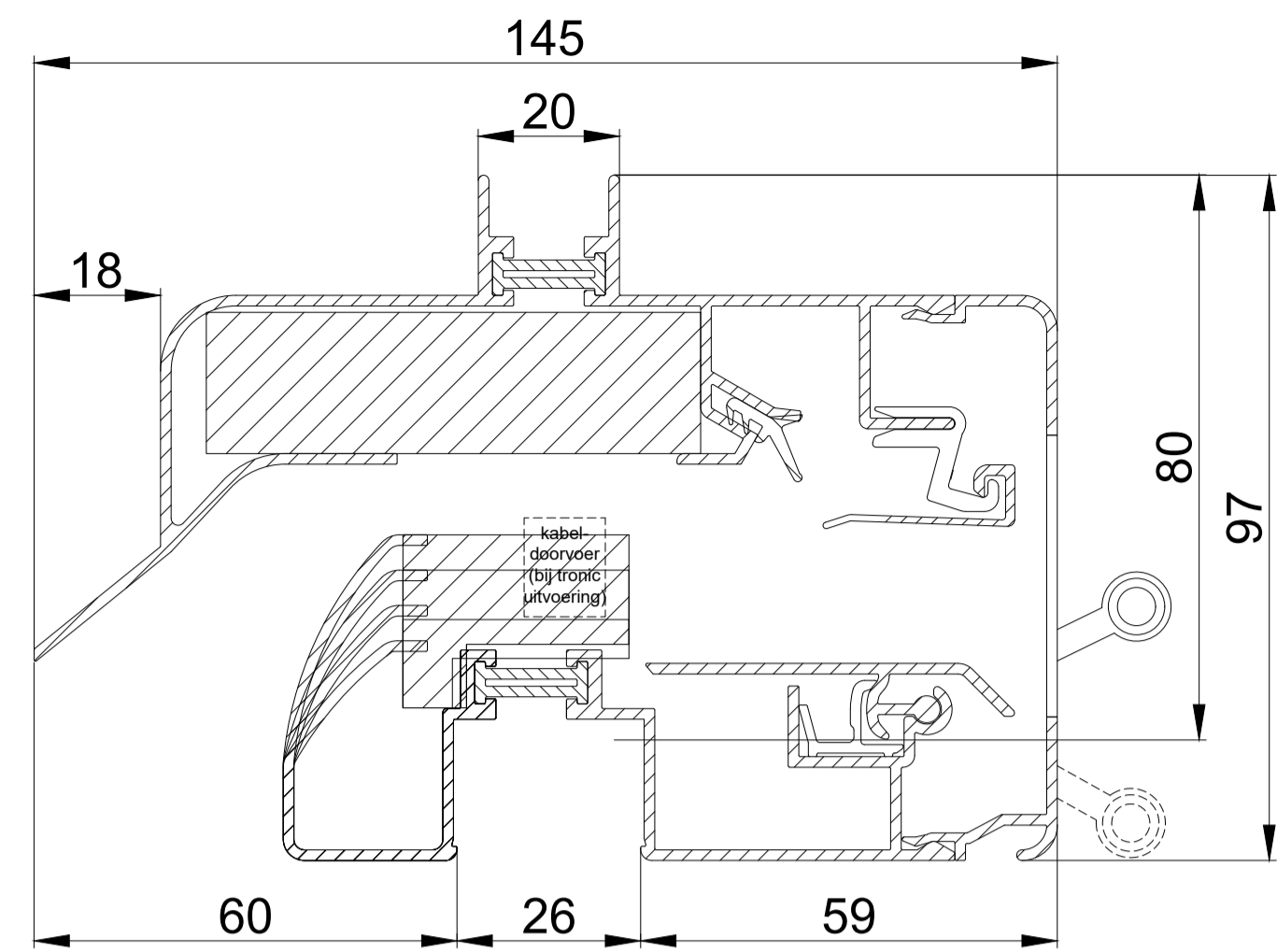
Glasmax 'ZR' / GG26
