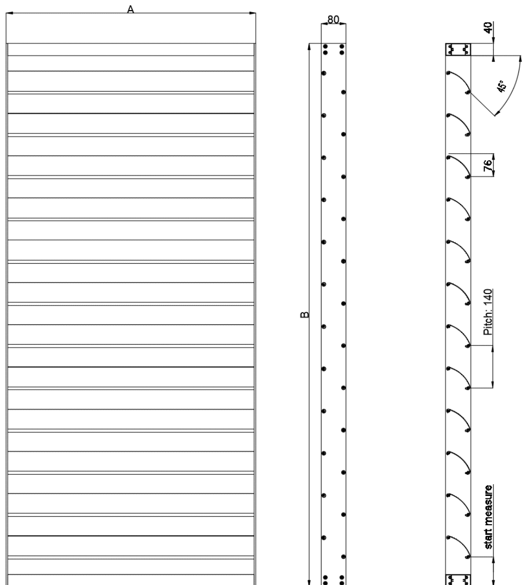
SECTION
