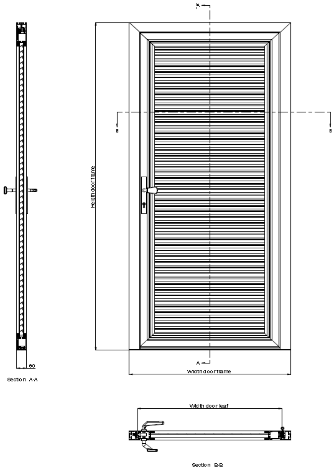
Section B-B
