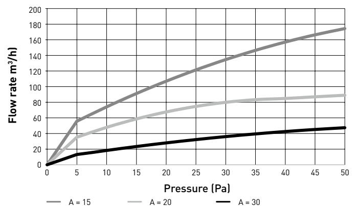
Pressure / flow curve DucoVent Basic
